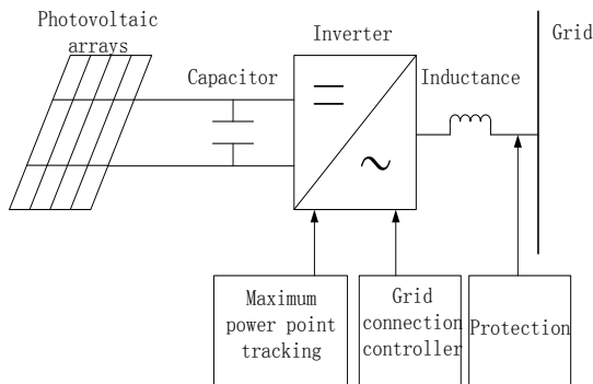
Fig. 1. PV generation system structure
