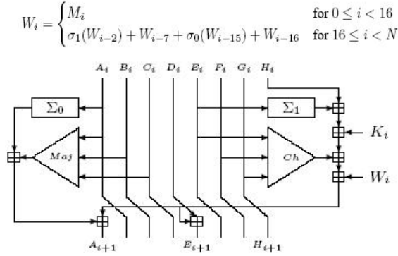
Figure 1: One step of the SHA-256 compression function
