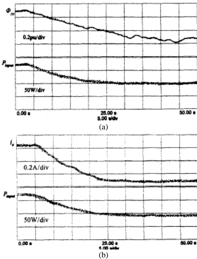
Fig. 9 Loss minimization on process in the 1-hp drive when the controlled variable IS (a) the input power and (b) the stator current
