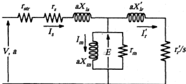
Fig.3 Per unit induction motor equivalent circuit
