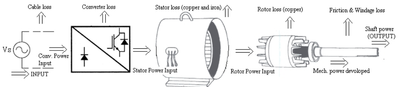
Fig. 1 Losses in the induction motor drive system
