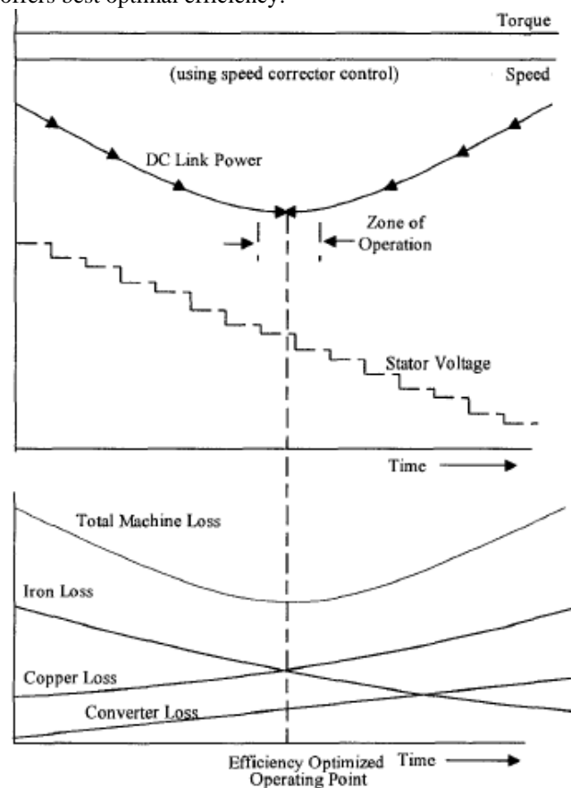
Fig. 10 Perturbation Optimizing Control
