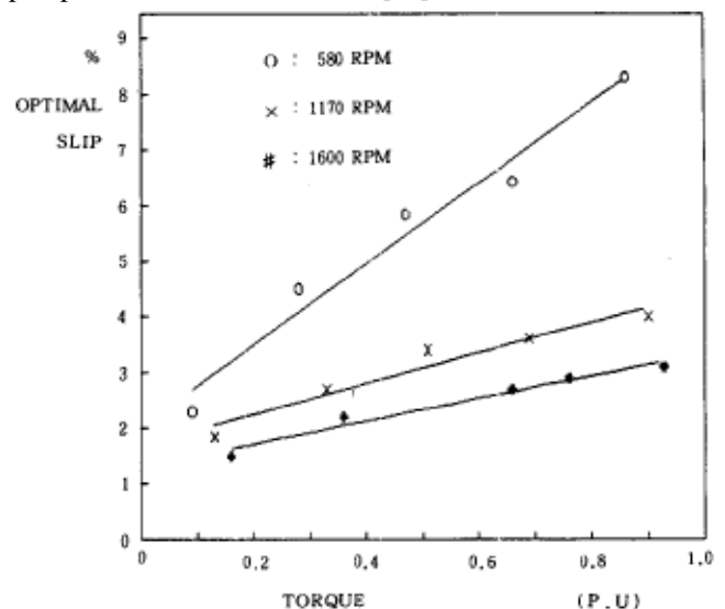
Fig. 4 Optimal slip versus torque at various speed
