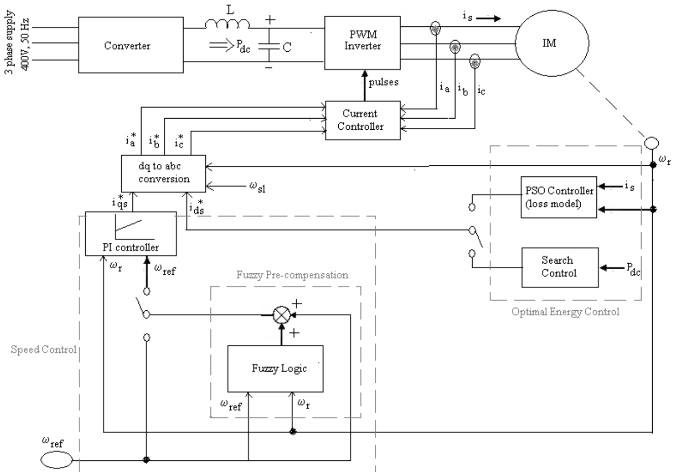
Fig. 2. Block diagram of optimal energy and speed control using PSO and fuzzy logic
