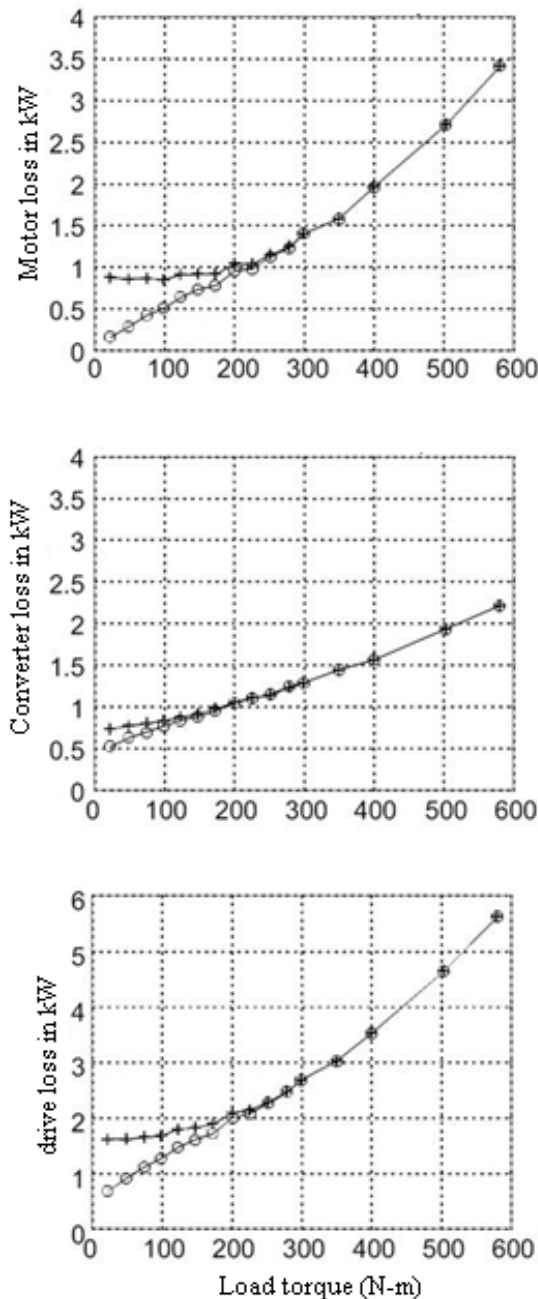
Fig. 5 Converter, drive and motor losses in 90 kW motor at 900 rpm speed.
