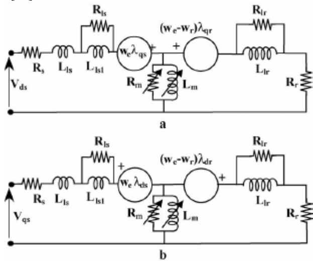
Fig. 7 Modified equivalent circuits for induction motor dynamic model. (a) d-axis equivalent circuit (b) q-axis equivalent circuit
