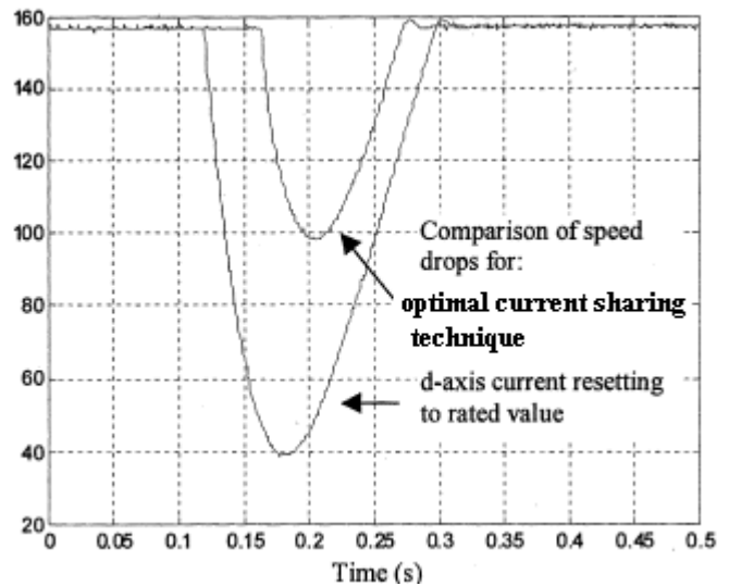
Fig. 8 Speed drops for the 2.2-kW induction motor drive (load torque stepped to 50 Nm)
